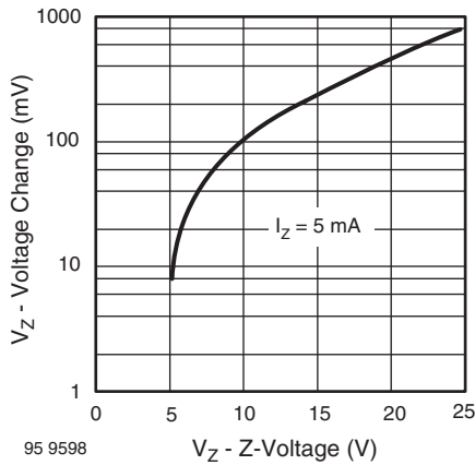
Fig. 2 - Typical Change of Working Voltage under Operating Conditions at T_{amb}=25^{\circ}\text{C}
