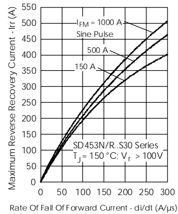
Fig. 23 - Recovery Current Characteristics
