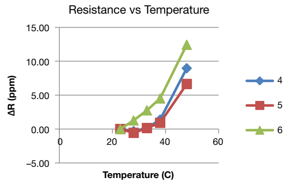
FIGURE 7—NOISE GENERATION—VISHAY FOIL RESISTOR VS. OTHER TECHNOLOGIES
