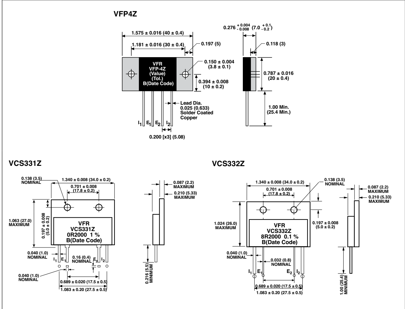
FIGURE 7—STANDARD IMPRINTING AND DIMENSIONS in inches (millimeters)
