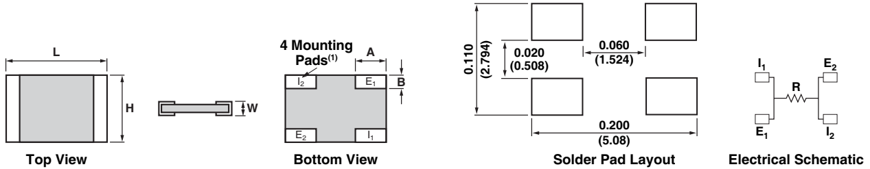
Figure 3 – Dimensions in inches (millimeters)
