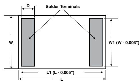
BOTTOM VIEW (showing terminals for mounting)
