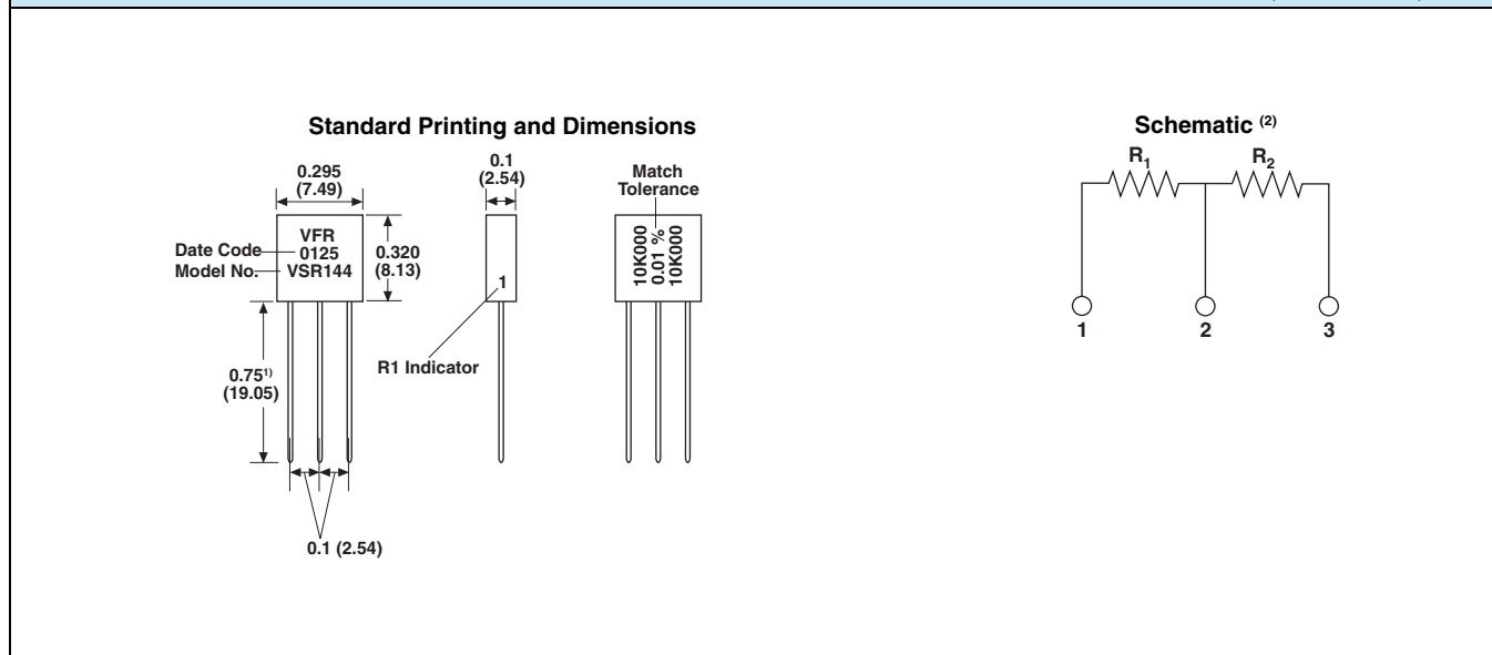
FIGURE 2 - MODEL VSR144 STANDARD PRINTING AND DIMENSIONS in inches (millimeters)
