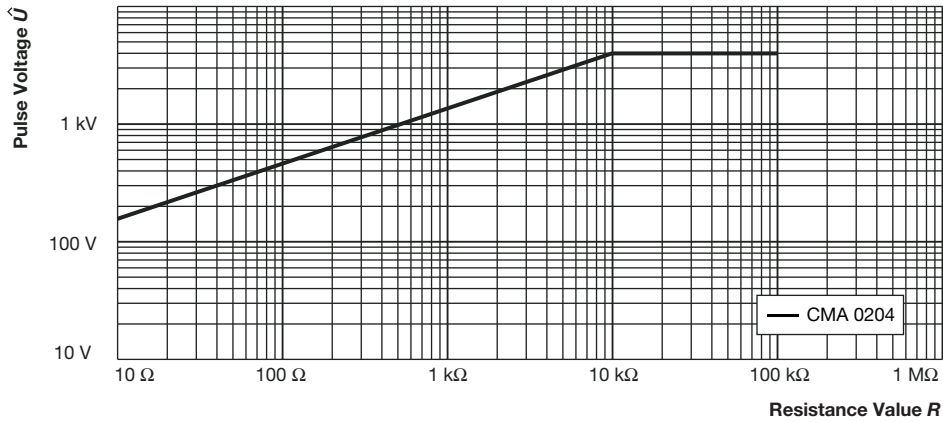
Pulse load rating in accordance with IEC 60115-1, 4.27; 1,2 μs/50 μs; 5 pulses at 12 s intervals; for permissible resistance change \pm (0.5 \% R + 0.05 \Omega)
