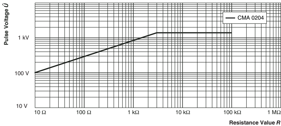
Pulse load rating in accordance with IEC 60115-1, 4.27; 10 μs/700 μs; 10 pulses at 1 minute intervals; for permissible resistance change \pm (0.5 \% R + 0.05 \Omega)
