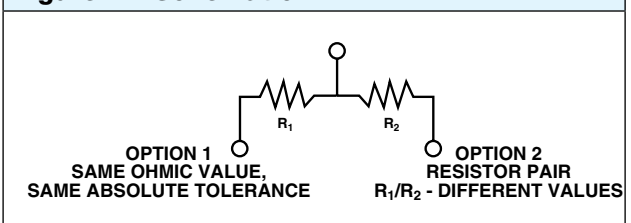
Figure 1 – Schematic
