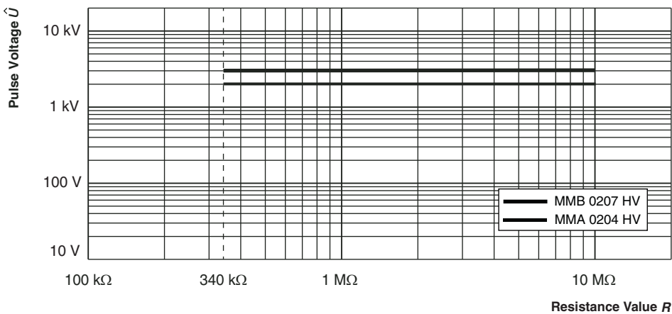
Pulse load rating in accordance with IEC 60 115-1, 4.27; 1.2 \mu s/50 \mu s; 5 pulses at 12 s intervals; for permissible resistance change (0.5 % R + 0.05 \Omega )
