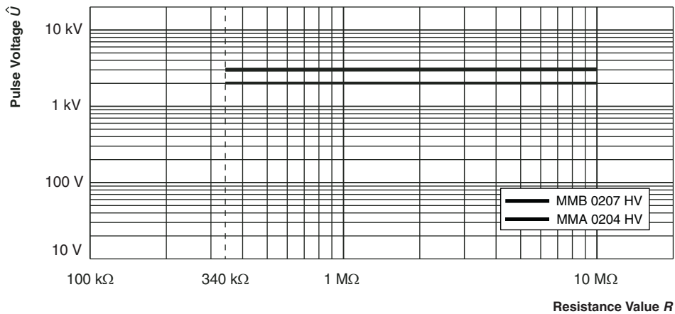
Pulse load rating in accordance with IEC 60115-1, 4.27; 10 \mu s/700 \mu s; 10 pulses at 1 minute intervals; for permissible resistance change (0.5 % R + 0.05 \Omega )
