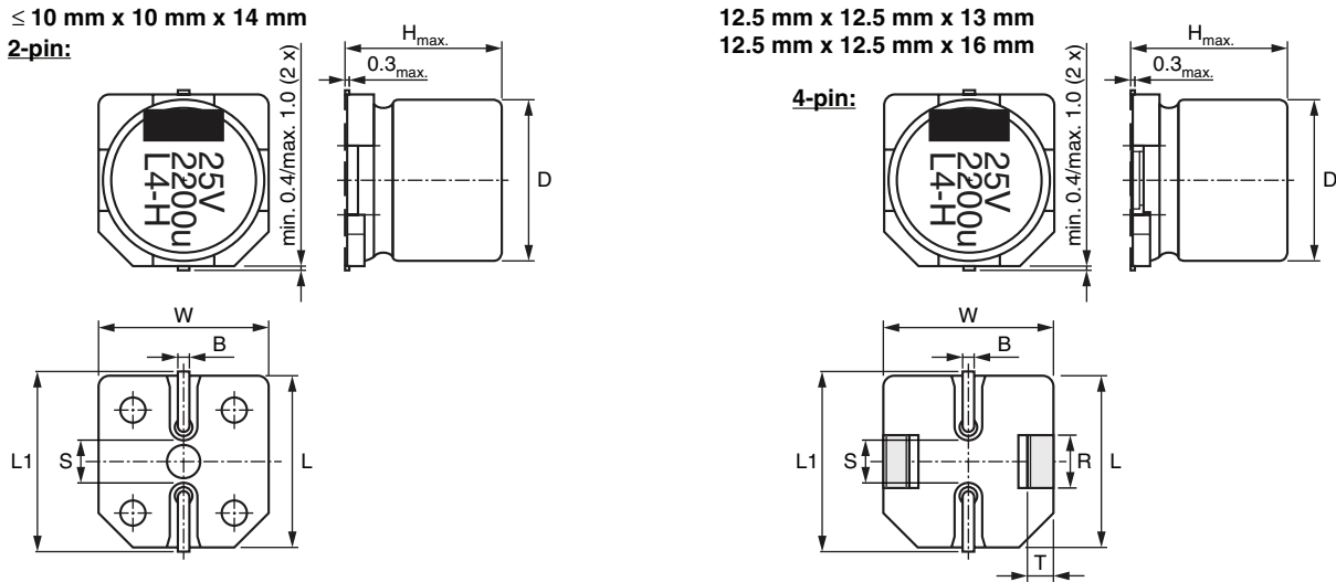
Fig.2 Dimensional outline
