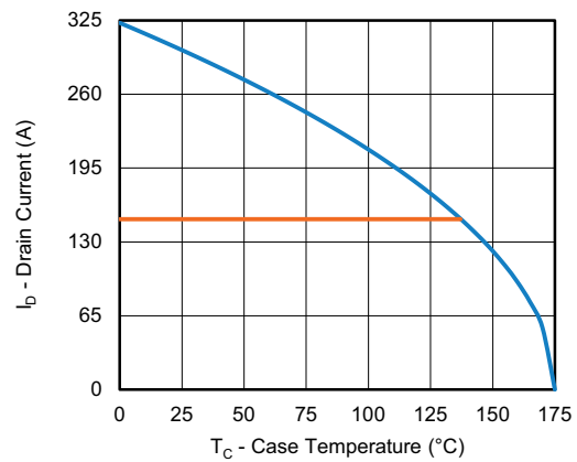
Current De-rating
