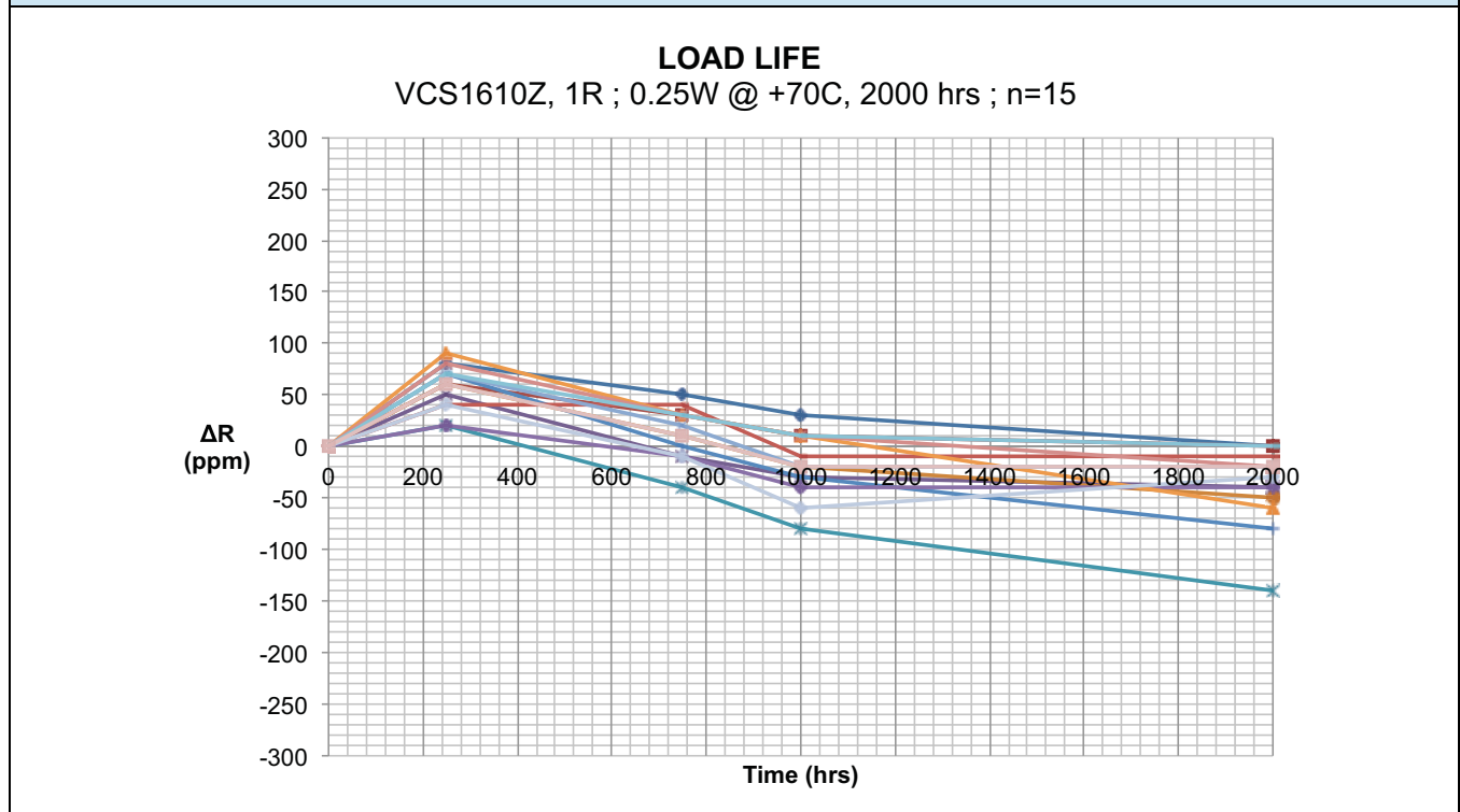
FIGURE 6 - LOAD LIFE
