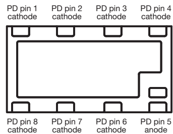
Pinning bottom view
