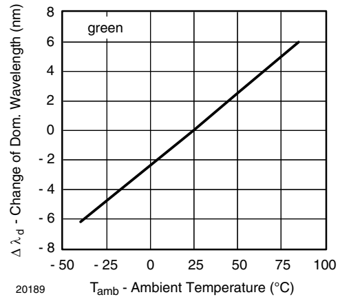
Fig. 12 - Change of Dominant Wavelength vs. Ambient Temperature
