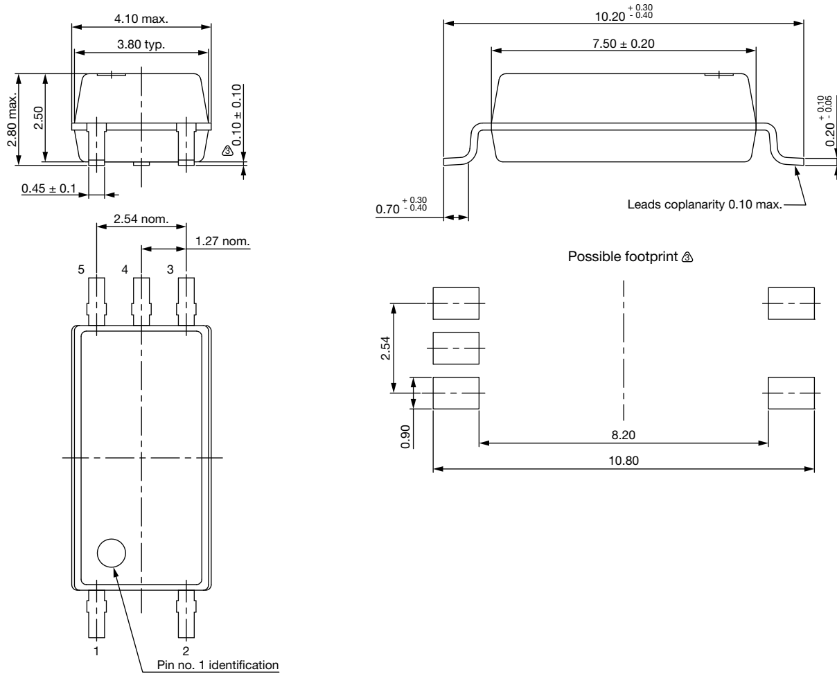
Fig. 20 - Package Drawing
