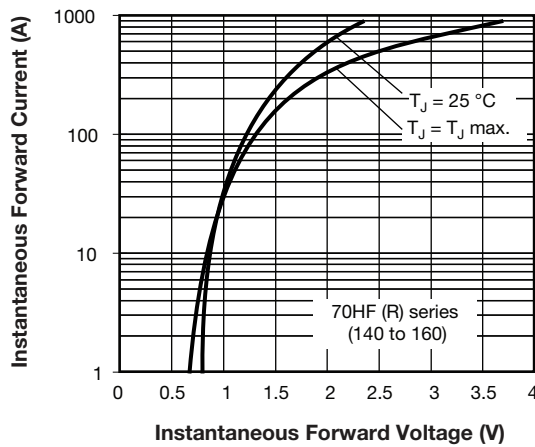
Fig. 13 - Forward Voltage Drop Characteristics
