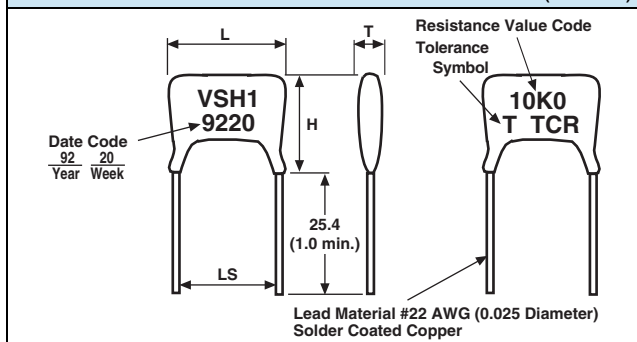
FIGURE 1 - STANDARD IMPRINTING AND DIMENSIONS in millimeters (inches)
