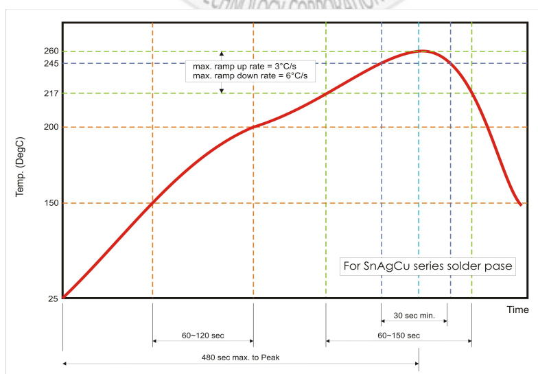
Fig 3. Infrared soldering profile for Chip Resistors WR02X SMT process with SnAgCu series solder paste
