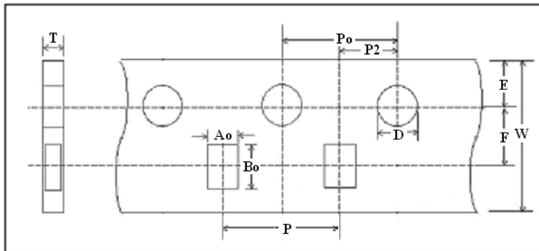
Taping Dimension
