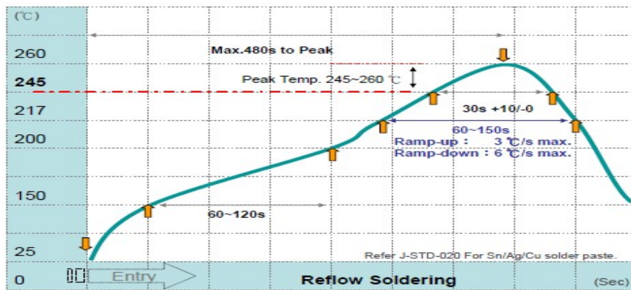
Fig 3. Infrared soldering profile for Chip Resistors WW25A
