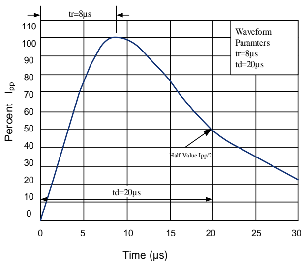
Figure 5: 8/20µs Pulse Waveform
