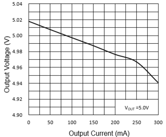
Output Voltage vs. Output Current
