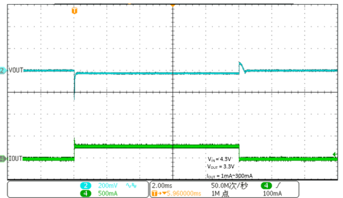
Load Transient
