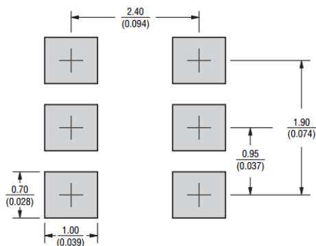
DIMENSIONS = MILLIMETERS (INCHES)
