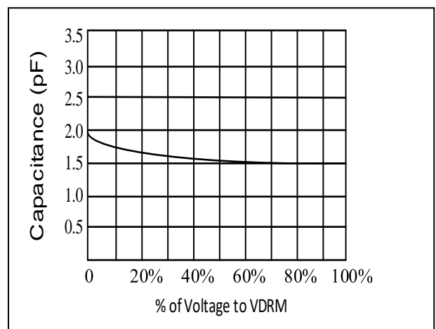
Typical capacitance against line voltage (without external bias)
