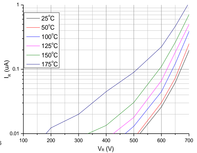
Fig.2-Reverse Characteristics
