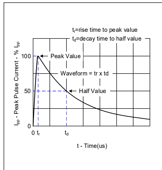
t_r X t_d Pulse Waveform
