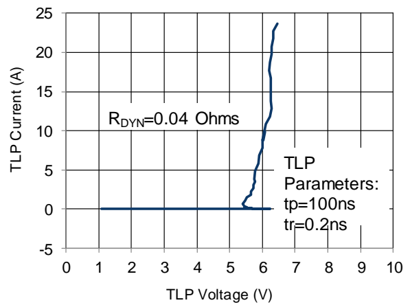
Figure 6: TLP Curve
