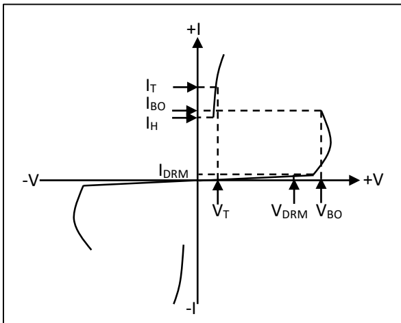
V-I Characteristics
