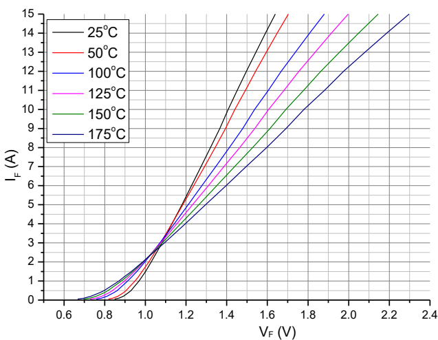
Fig.1-Forward Characteristics
