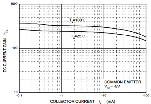
Figure 2. h FE vs. I C
