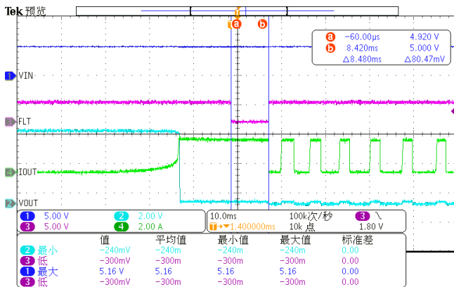
Over Current Conditions Indicated by \overline{FLT}
