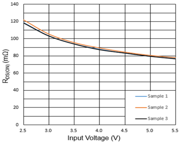
R DS(ON) (mΩ) vs. Supply Voltage
