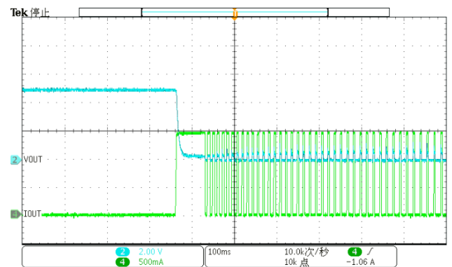
Short Current Response & Thermal Shutdown
