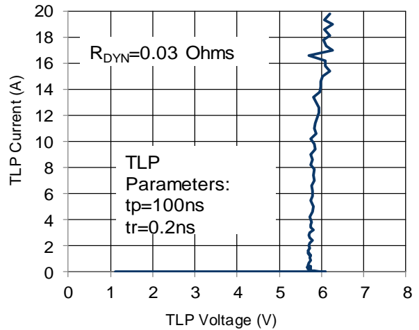
Figure 6: TLP Curve
