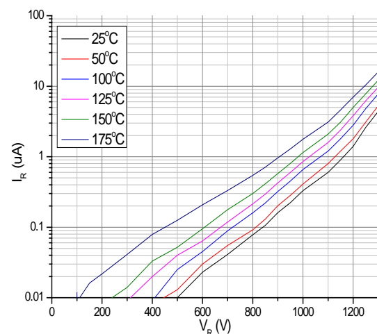
Fig.2-Reverse Characteristics
