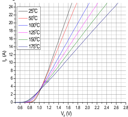
Fig.1-Forward Characteristics
