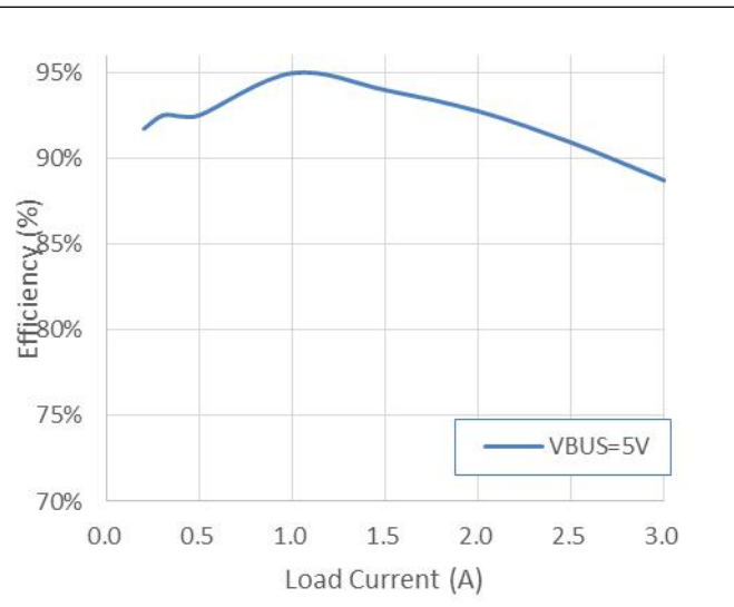
Figure 2. System Efficiency vs System Load Current
