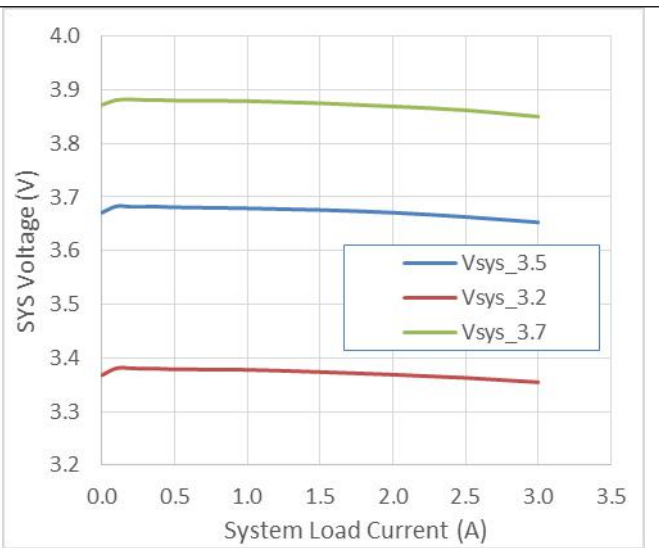
Figure 4. SYS Voltage Regulation vs System Load Current
