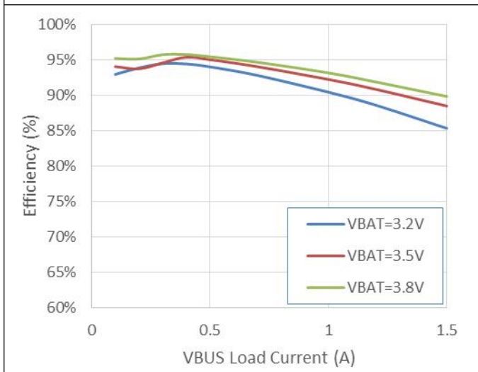
Figure 3. Boost Mode Efficiency vs VBUS Load Current
