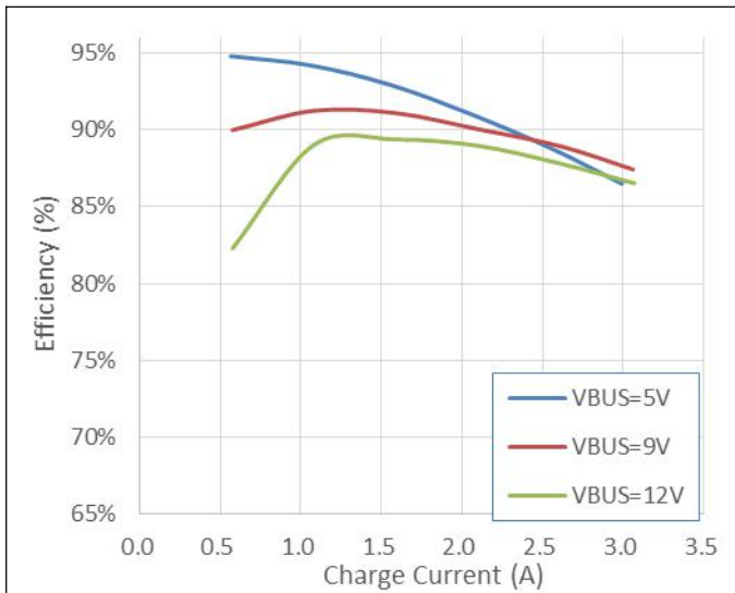
Figure 1. Charge Efficiency vs Charge Current
