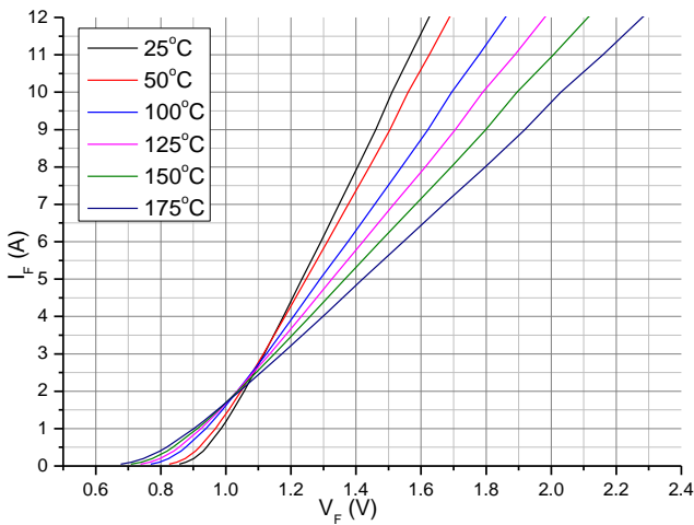
Fig.1-Forward Characteristics
