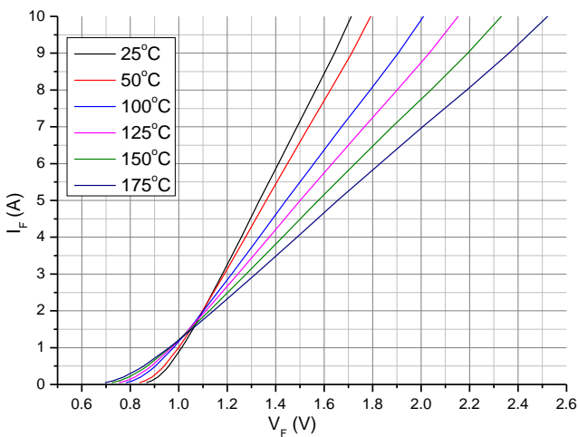
Fig.1-Forward Characteristics
