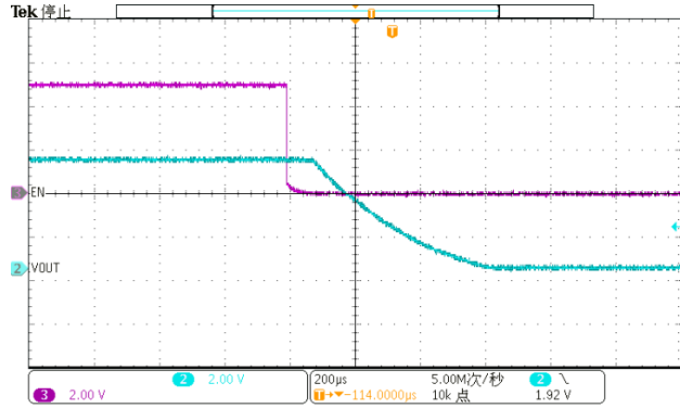
Turn Off Response
