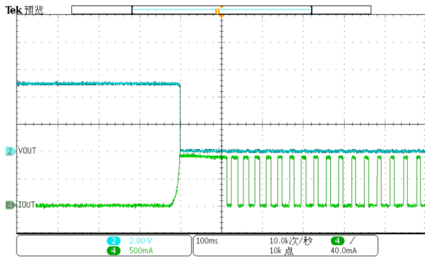
Short Current Response & Thermal Shutdown
