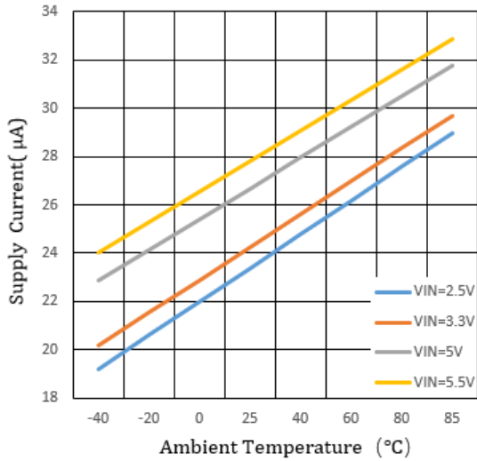
Quiescent Supply Current vs. Ambient Temperature
