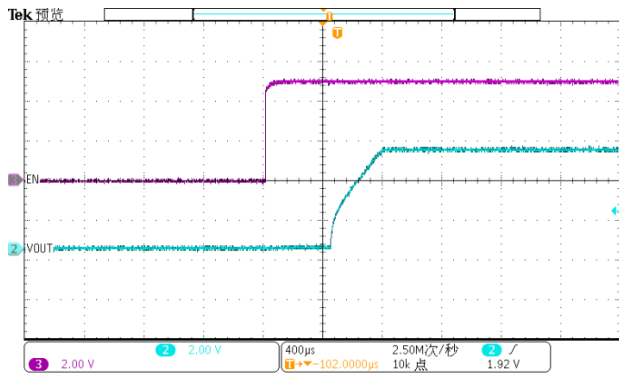
Turn On Response
