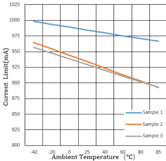
Current-Limit Threshold vs. Ambient Temperature
