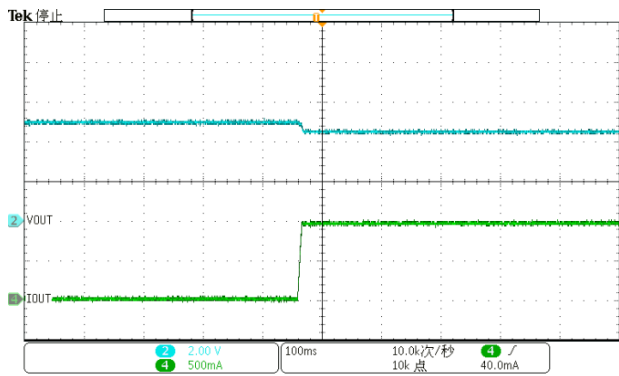
Overload Current-limit
