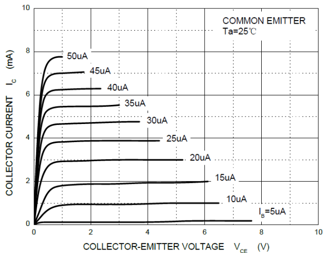
Figure 1. Static Characteristics
