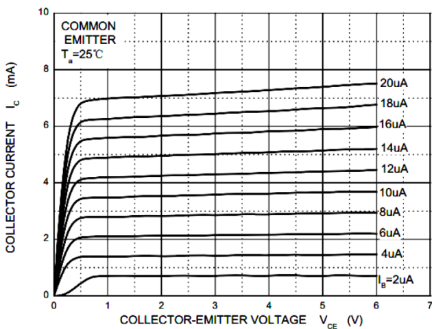
Figure 1. Static Characteristics
