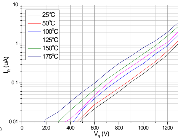
Fig.2-Reverse Characteristics
