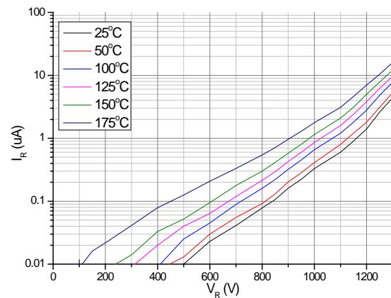
Fig.2-Reverse Characteristics
