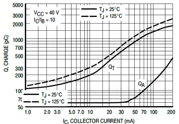
Figure 2. Charge Data
