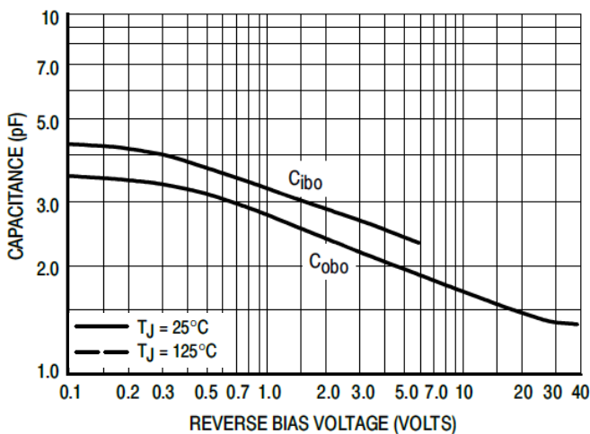
Figure 1. Capacitance
