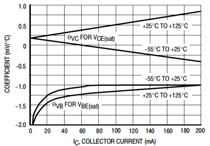
Figure 6. Temperature Coefficients
