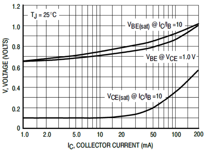
Figure 5. "ON" Voltages
