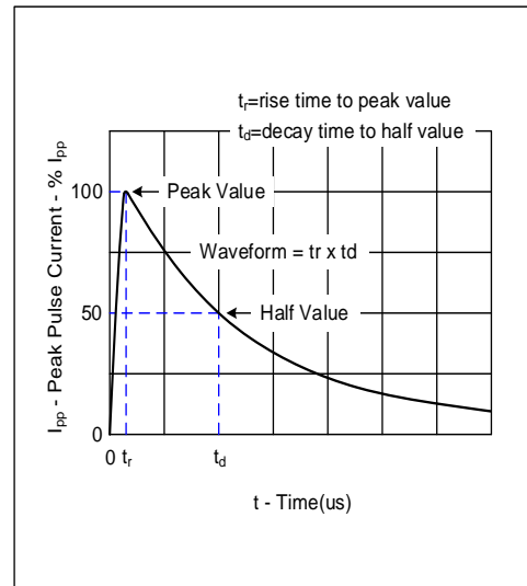
t r X t d Pulse Waveform
