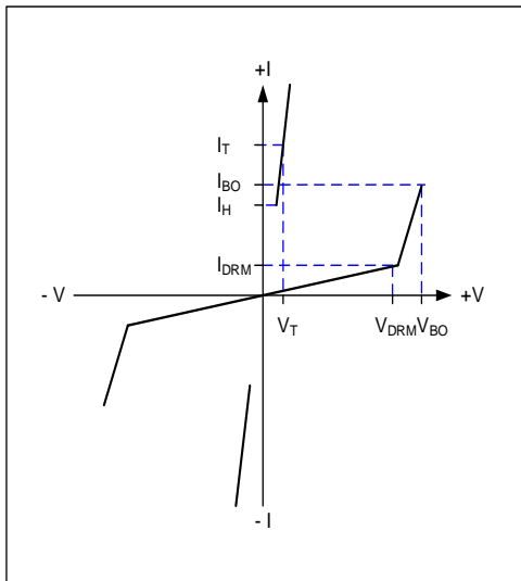
V - I Characteristics
