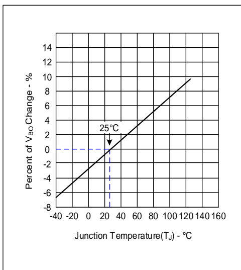
Normalized V BO Change versus Junction Temperature
