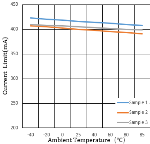
Current-Limit Threshold vs. Ambient Temperature (open R SET )
