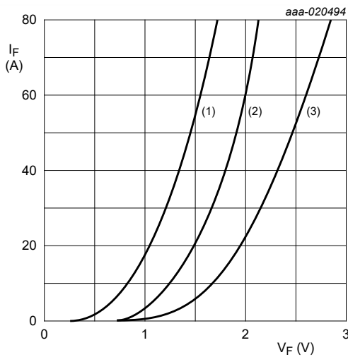
V_o = 1.994\text{ V}; R_s = 0.002\ \Omega (1) T_j = 150\text{ }^\circ\text{C}; typical values (2) T_j = 150\text{ }^\circ\text{C}; maximum values (3) T_j = 25\text{ }^\circ\text{C}; maximum values
