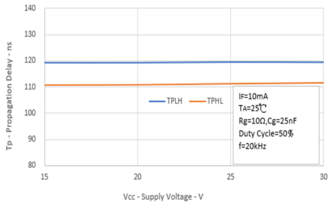
Fig.8 Propagation Delays vs. VCC
