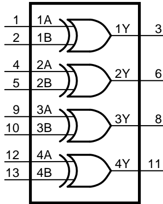
Figure 1. Logic symbol
