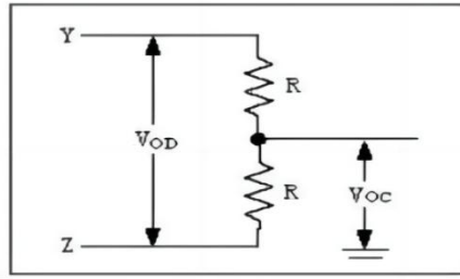
Figure 4: Drive DC test load
