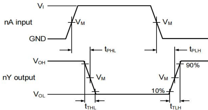
Figure 5. Input to output propagation delays
