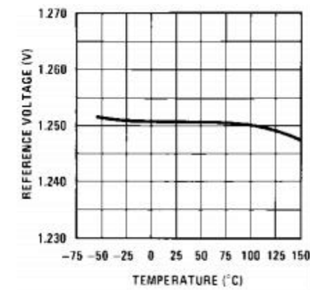
Figure 5. Temperature Stability
