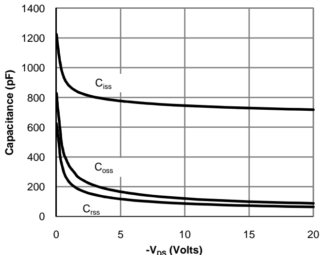
Figure 8: Capacitance Characteristics
